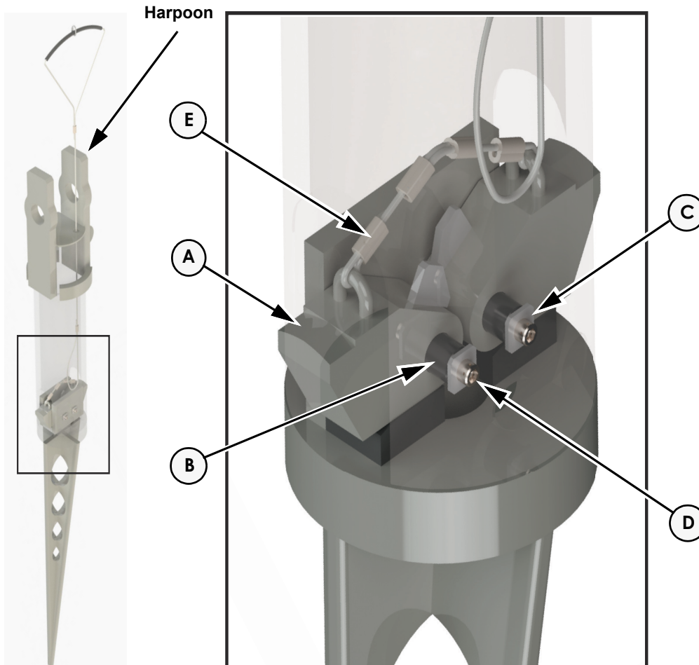
Figure 1: Harpoon latch components
